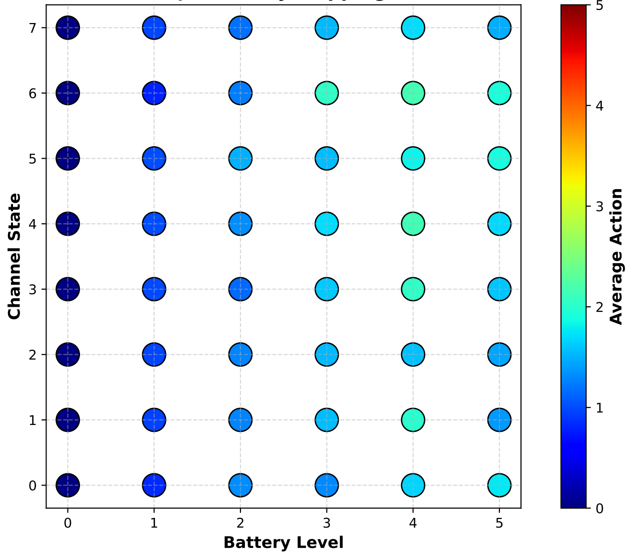
JAL: Policy Mapping
